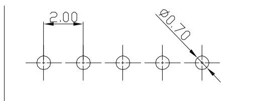
P. C. B LAYOUT
