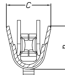
SECTION Z-Z
