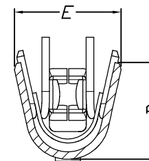
SECTION Y-Y
